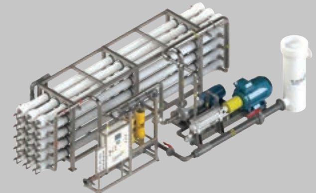
SWRO1350-EE
