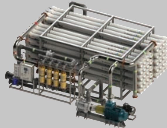
SWRO4000-EE
