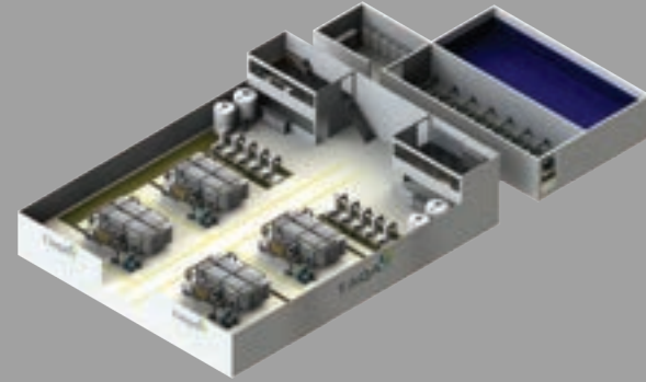
SWRO16,000-EE
